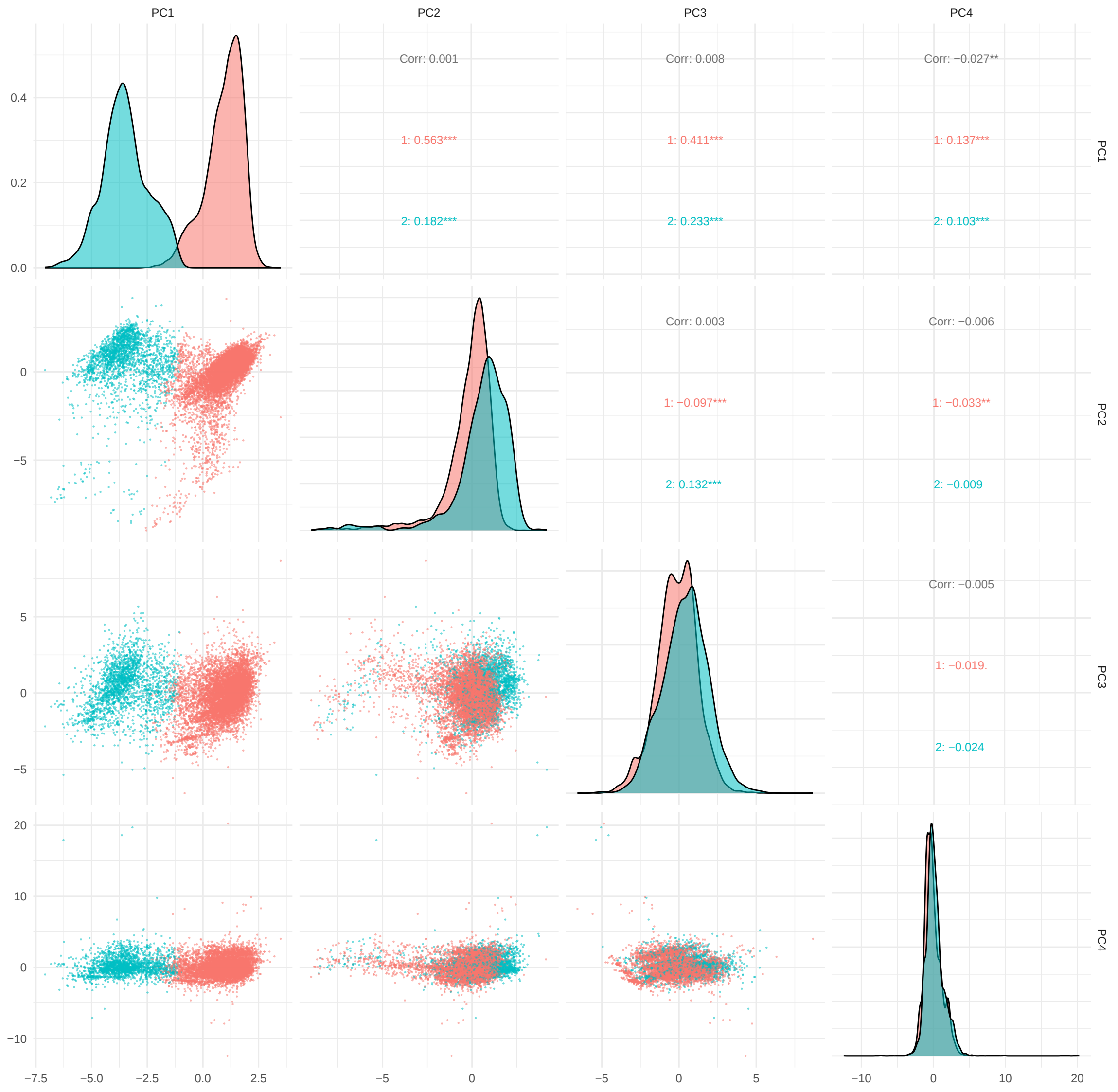
K-Means (k=) Cluster Separation across PC1–PC4
