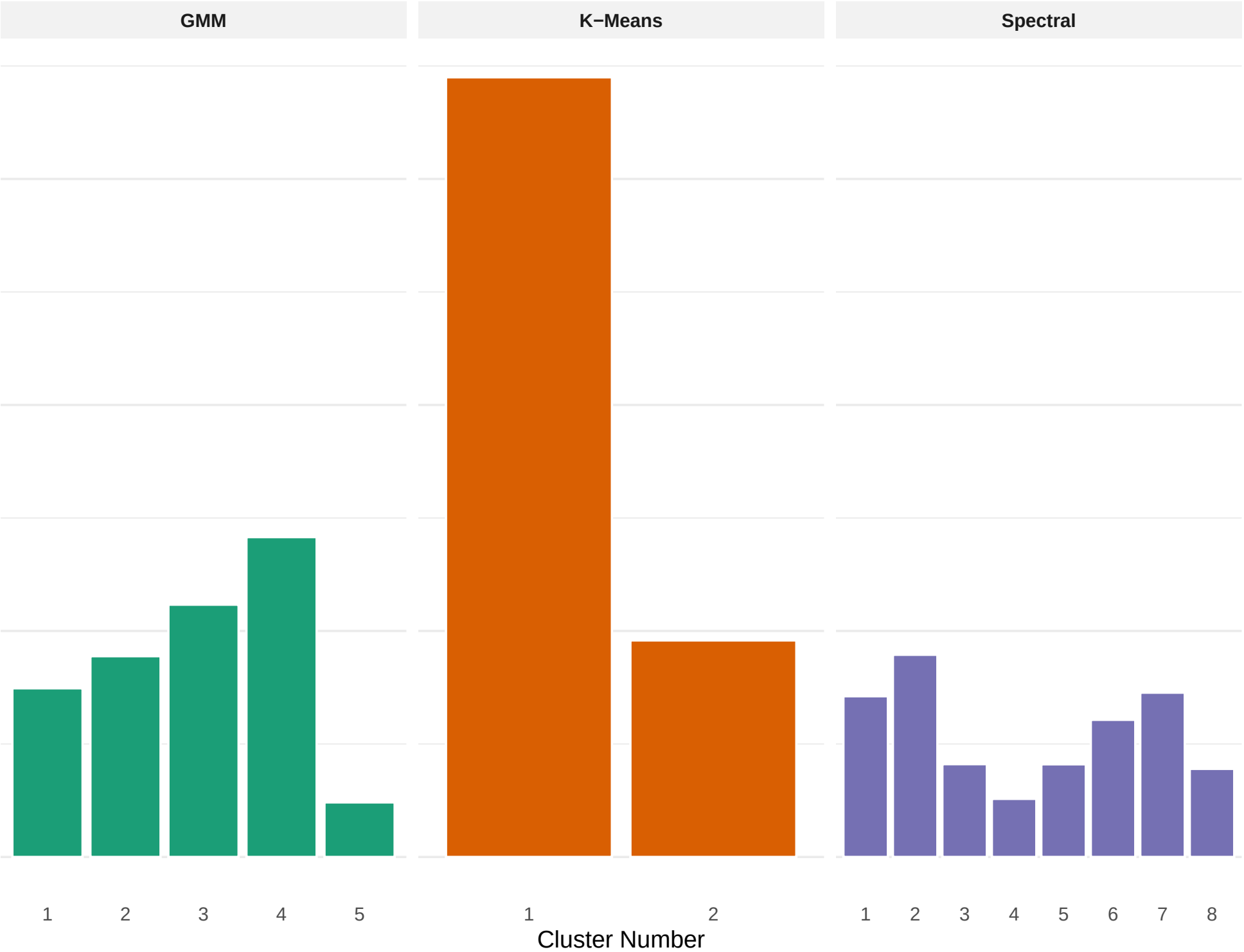
Observation Distribution across Cluster Models Comparative analysis of cluster assignments (N = 800k+ per model)
