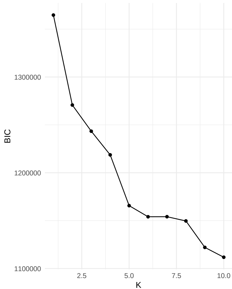
GMM Model Selection BIC vs Number of Clusters
