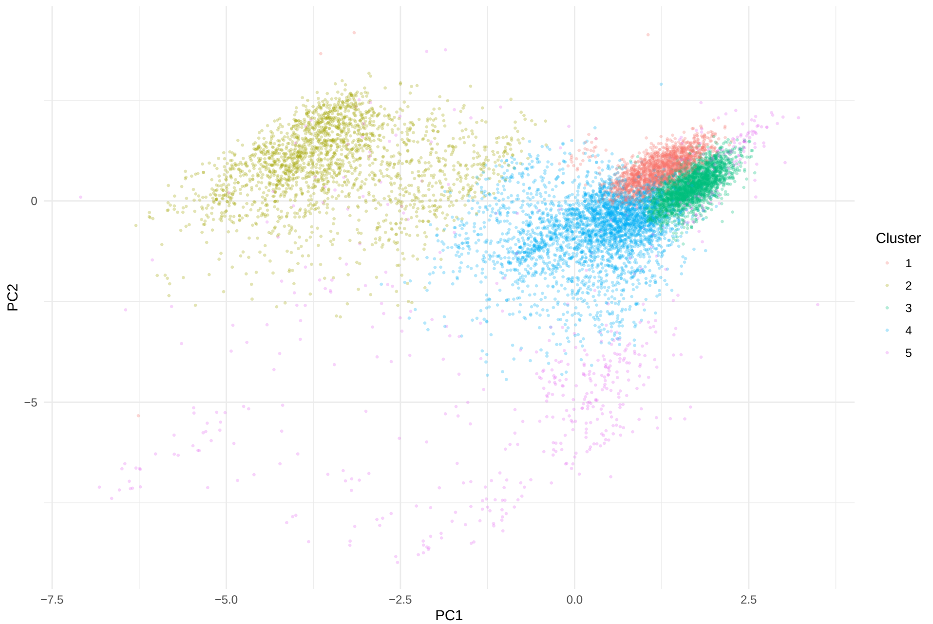
GMM: PC1 vs PC2 (Primary Dimensions)
