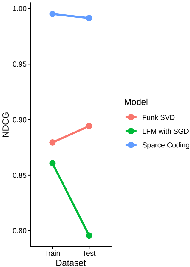
NDCG Generalization (Train vs Test)
