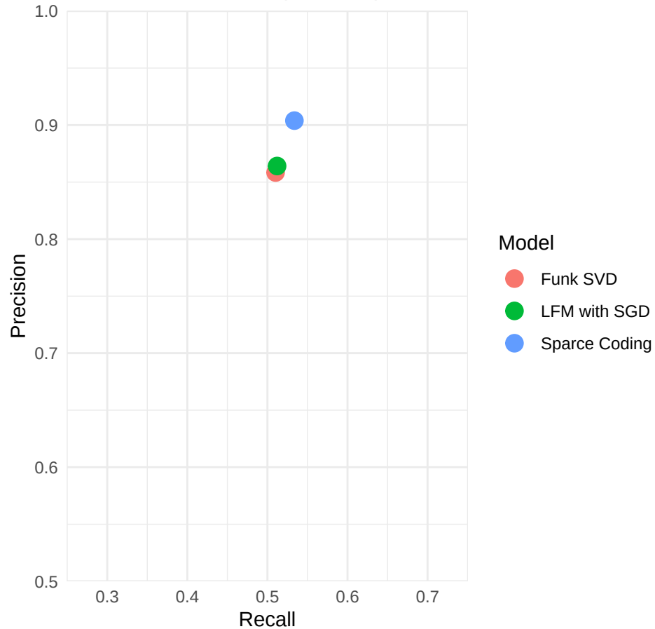
Precision vs Recall (Test Set)
