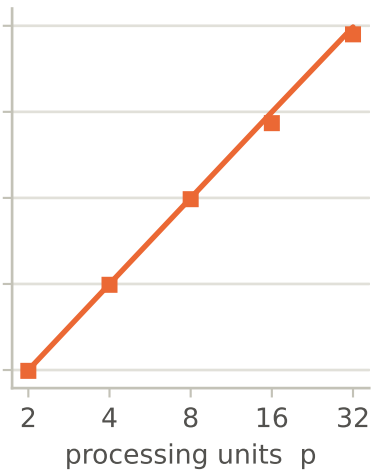
cyclic
