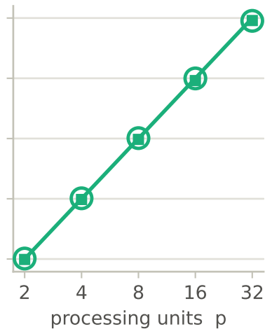
dynamic
