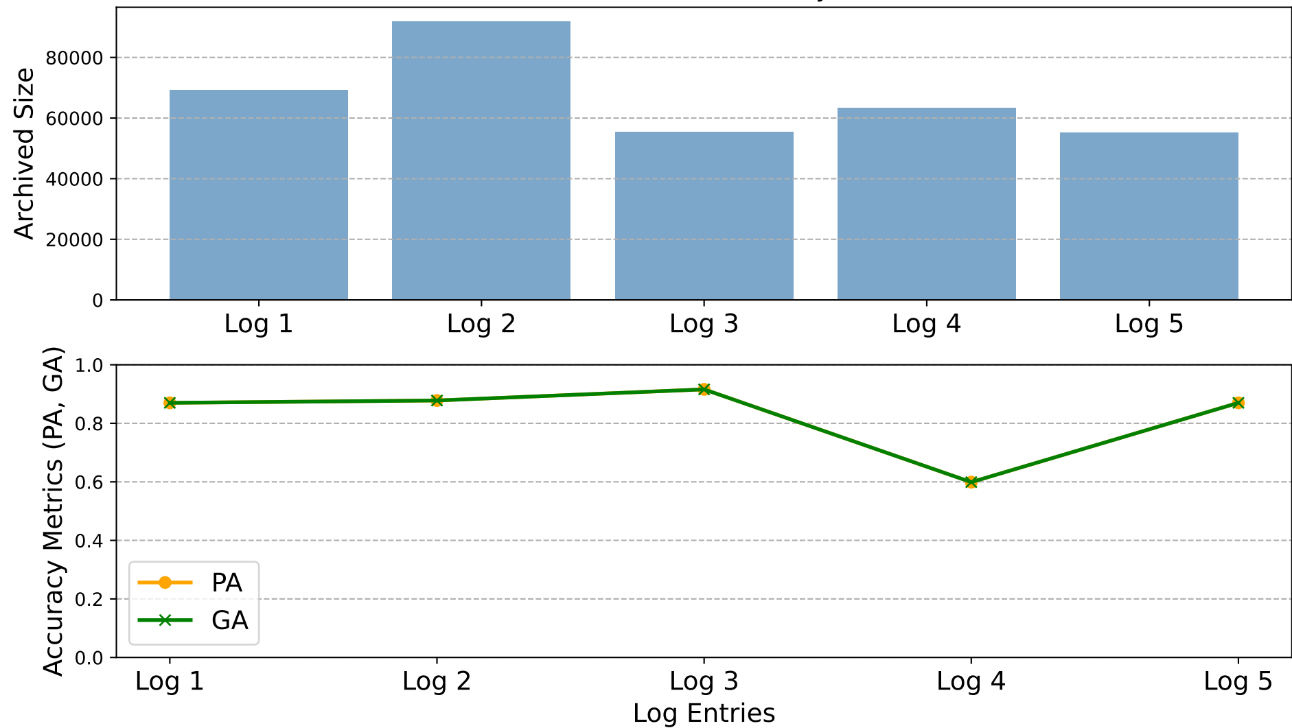
Archived Size and Accuracy Metrics
