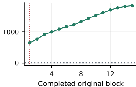
Hadoop (full)
