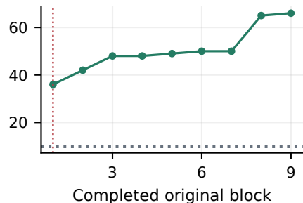
HealthApp (full)
