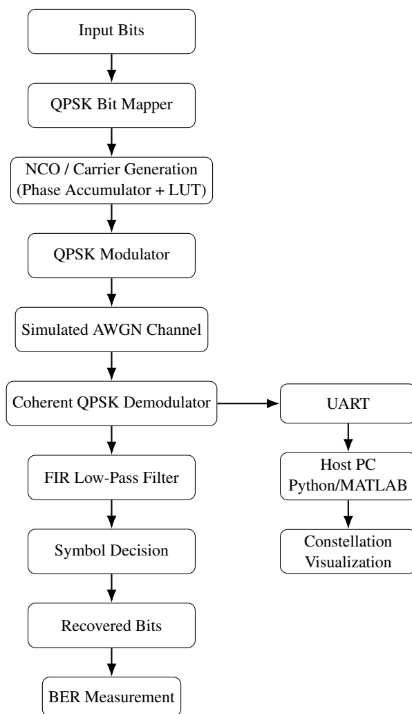
Figure 1. QPSK transmitter-channel-receiver block diagram
