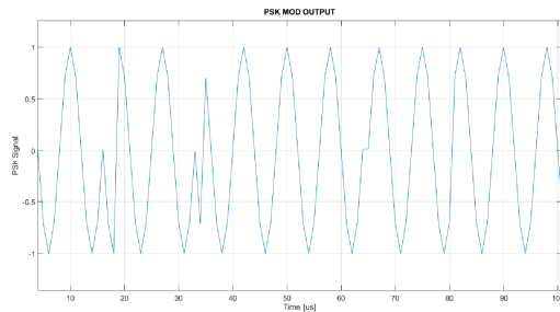
Fig. 9: QPSK implementation results.
