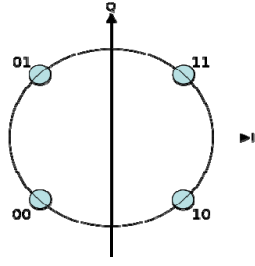
Fig.3: QPSK constellation diagram.
