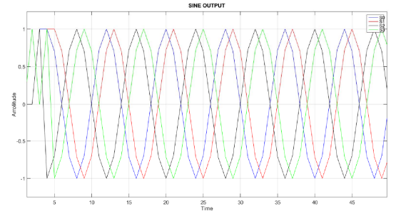
Fig. 8: The four generated sinusoids with 90-degree phase shift.
