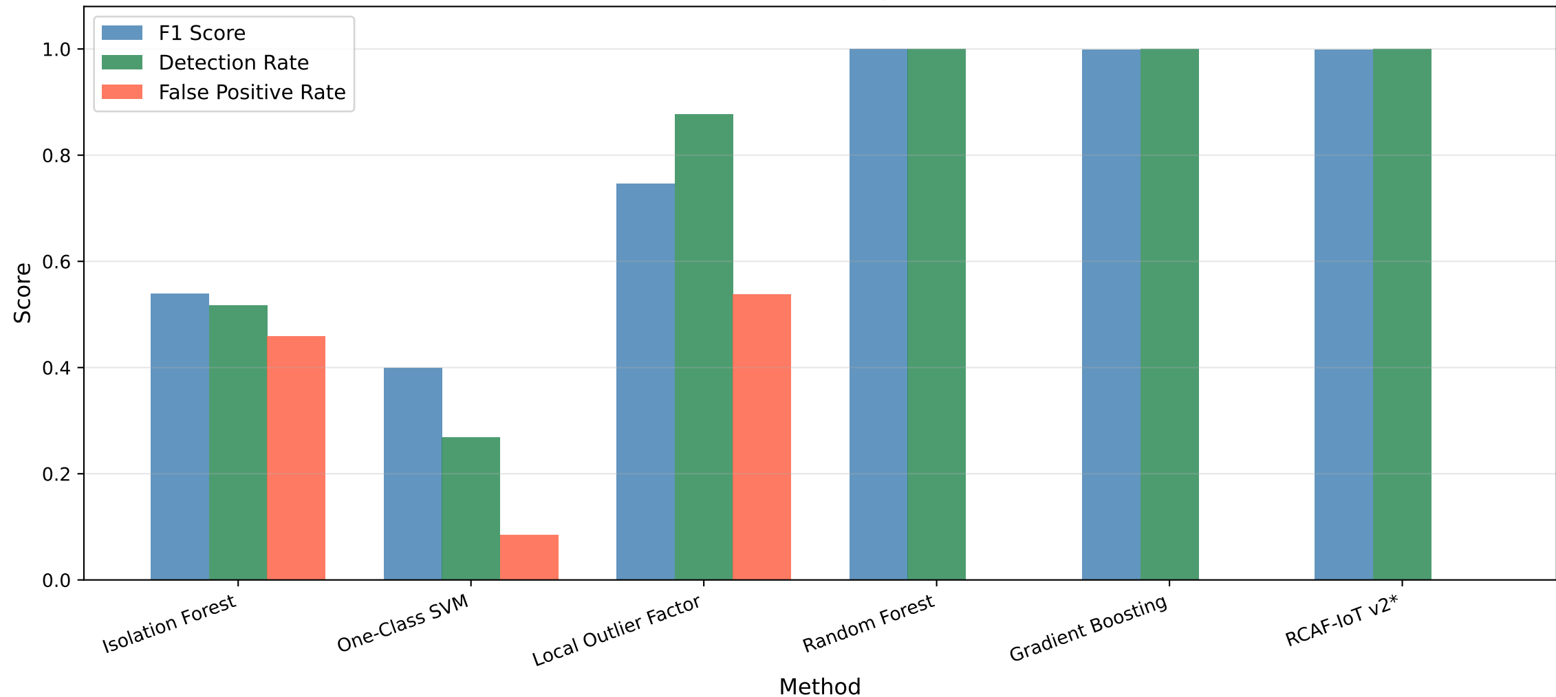
RCAF-IoT v2* vs Baseline Methods (*This Work — RF+GB+IF Hybrid Ensemble)
