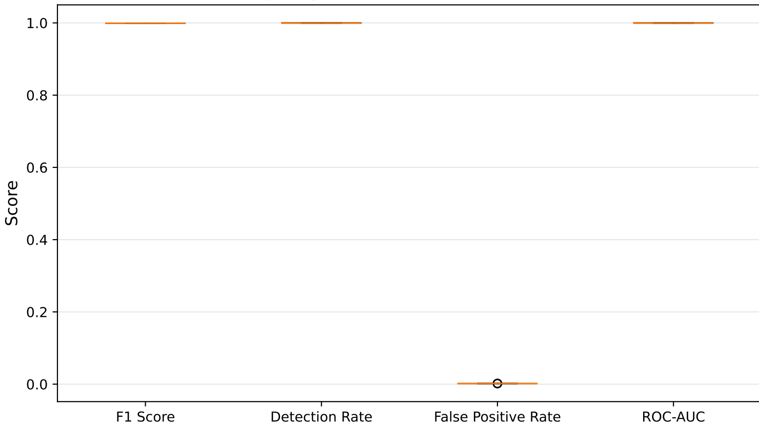
5-Fold Cross-Validation — RCAF-IoT v2 (Raspberry Pi 4 ARM Cortex-A72 @ 1.8GHz)
