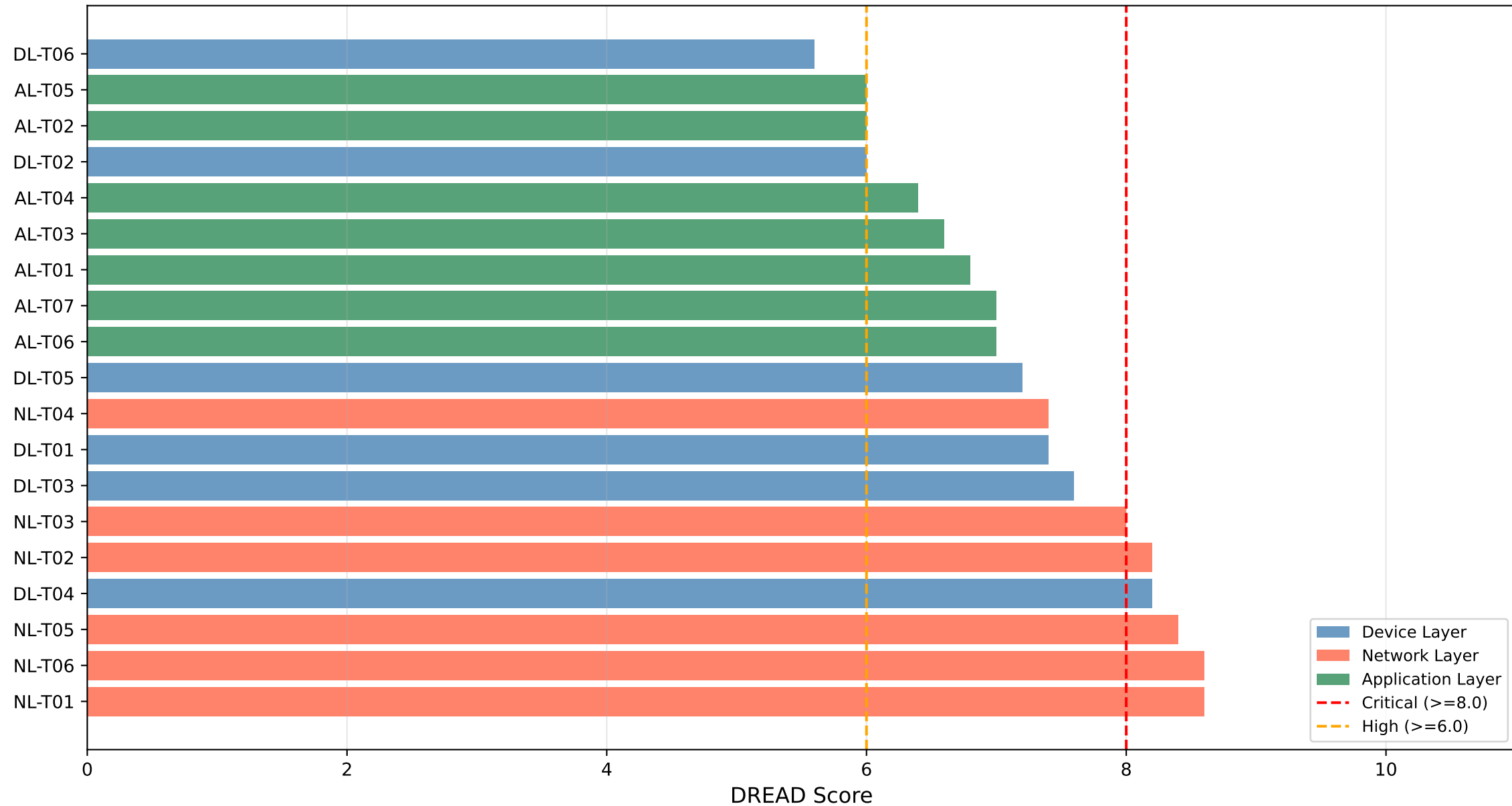
STRIDE-DREAD Threat Model Kinect v1 (Model 1473) + Raspberry Pi 4 — 19 Threat Vectors
