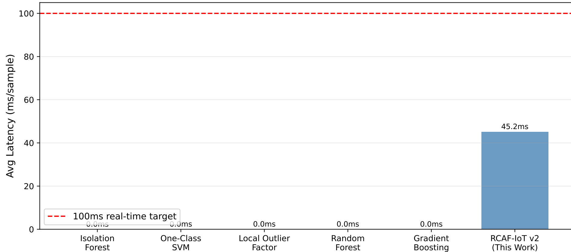
Inference Latency on Raspberry Pi 4 ARM Cortex-A72 (lower is better — 100ms = real-time threshold)
