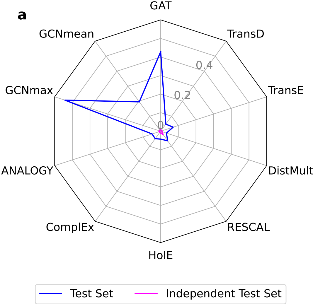
Indication MRR (Test Set vs Independent Test Set)
