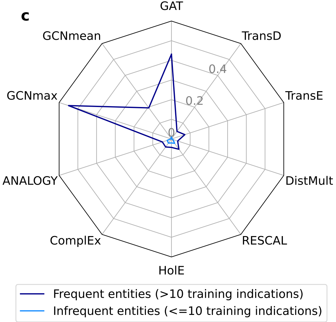
Test Set Indication MRR by entity frequency
