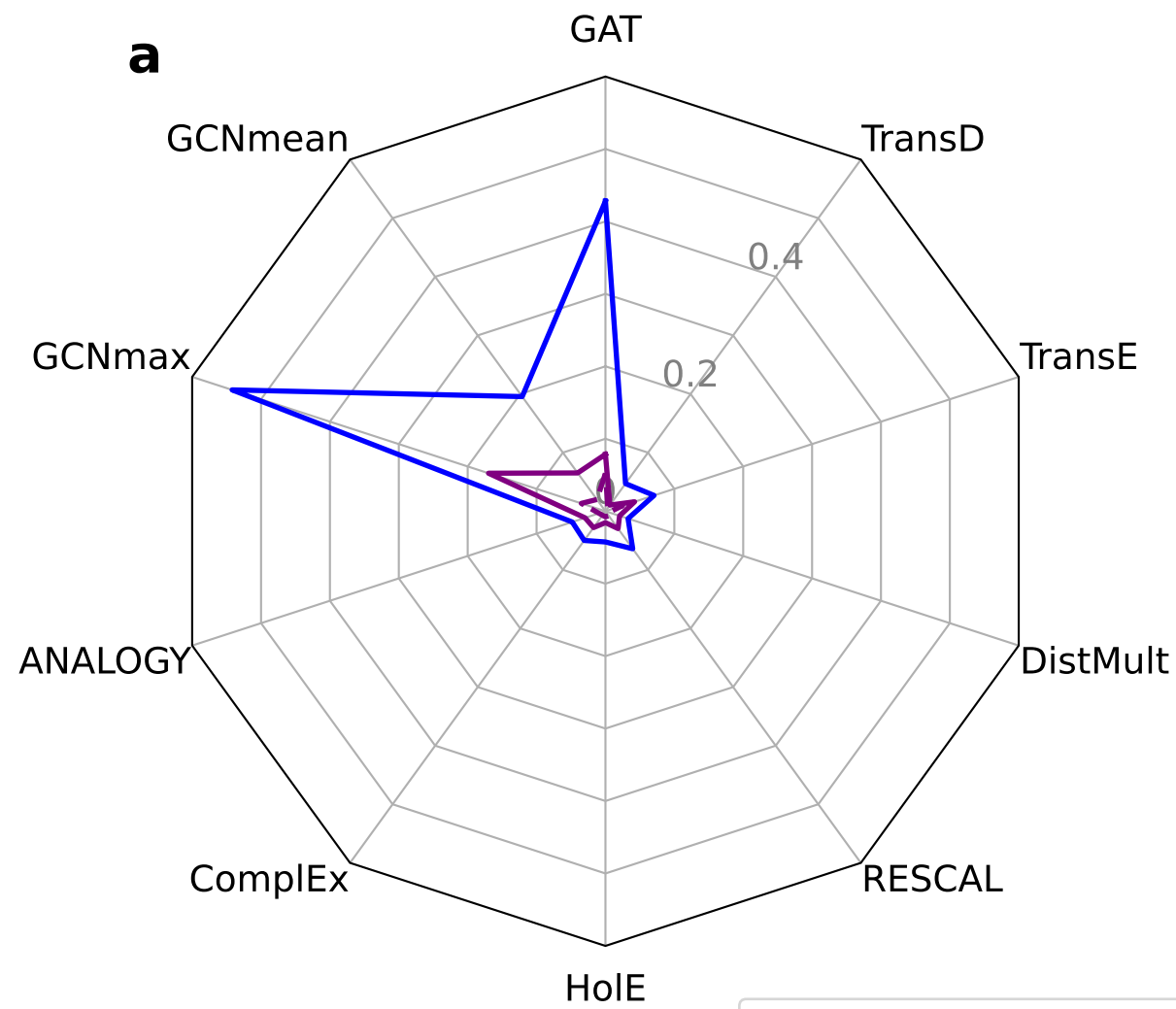
Test MRR
