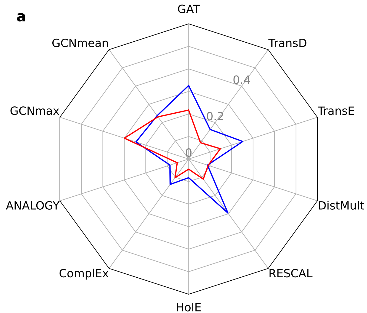
Indication MRR
