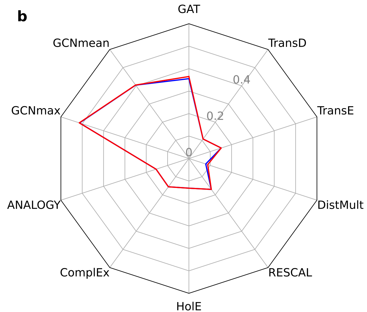
Global MRR
