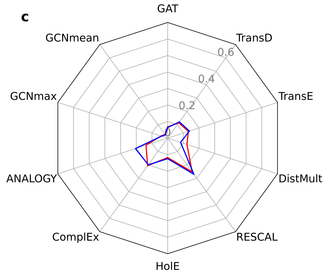
Indication MRR
