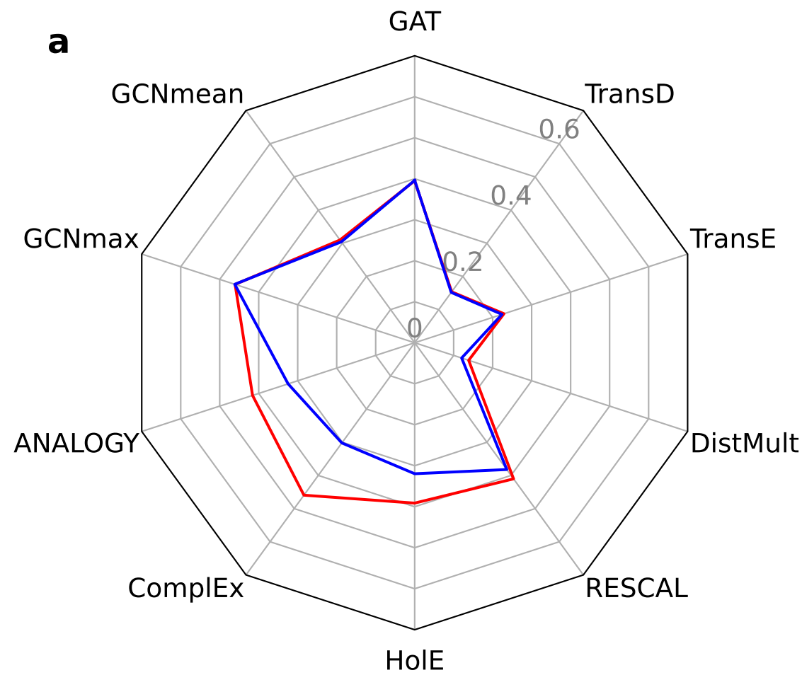
Global MRR
