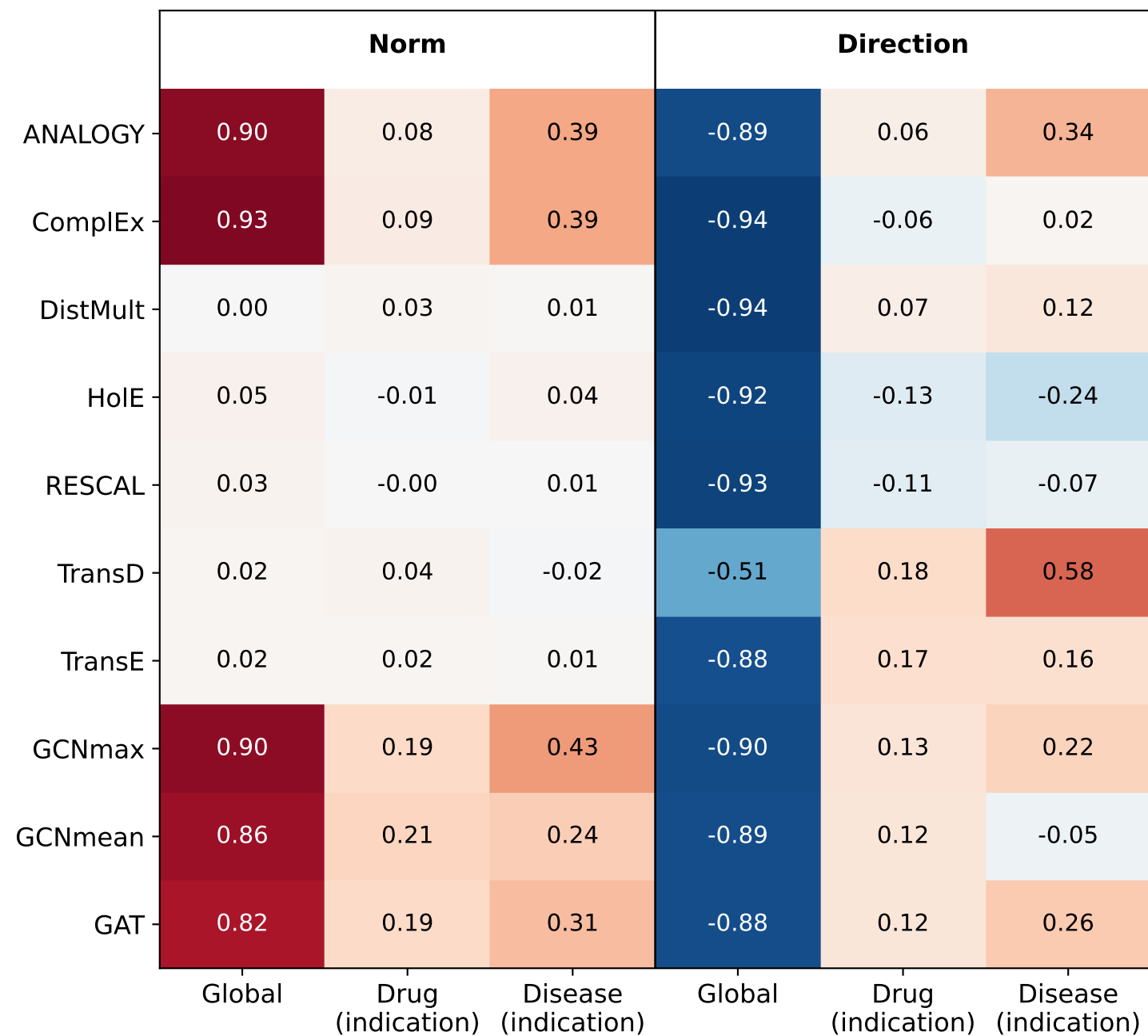
Original ShepherdKG
