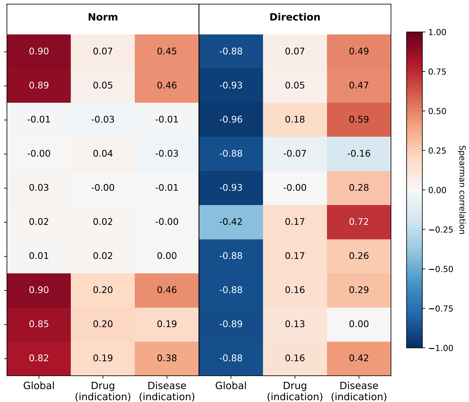
Permuted ShepherdKG
