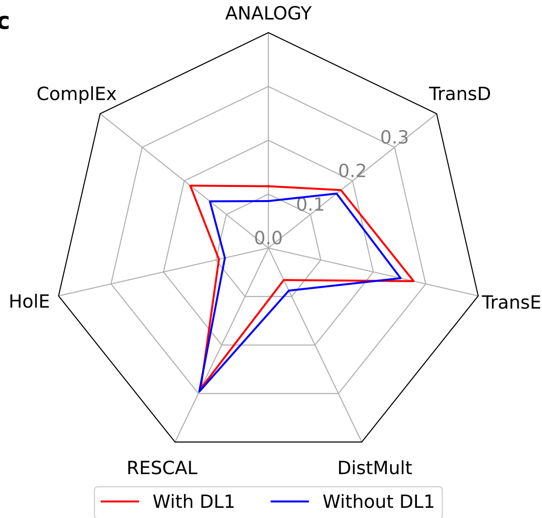
Indication MRR
