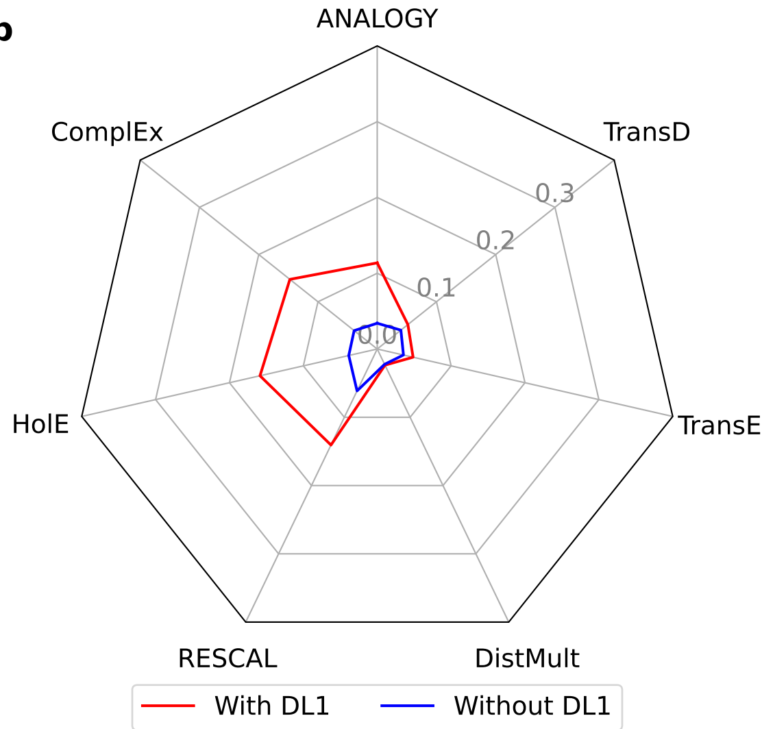
Redundant Relations MRR
