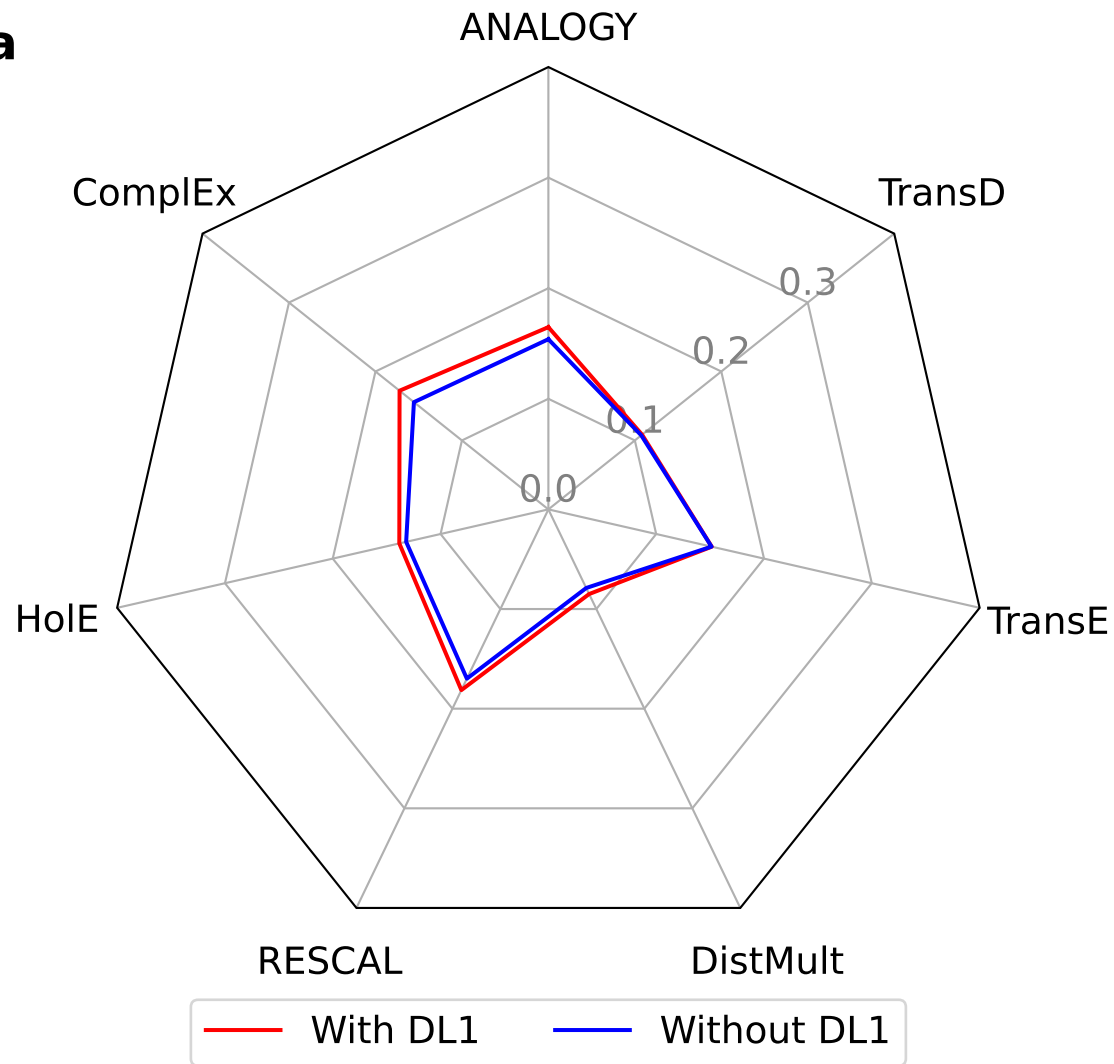
Global MRR
