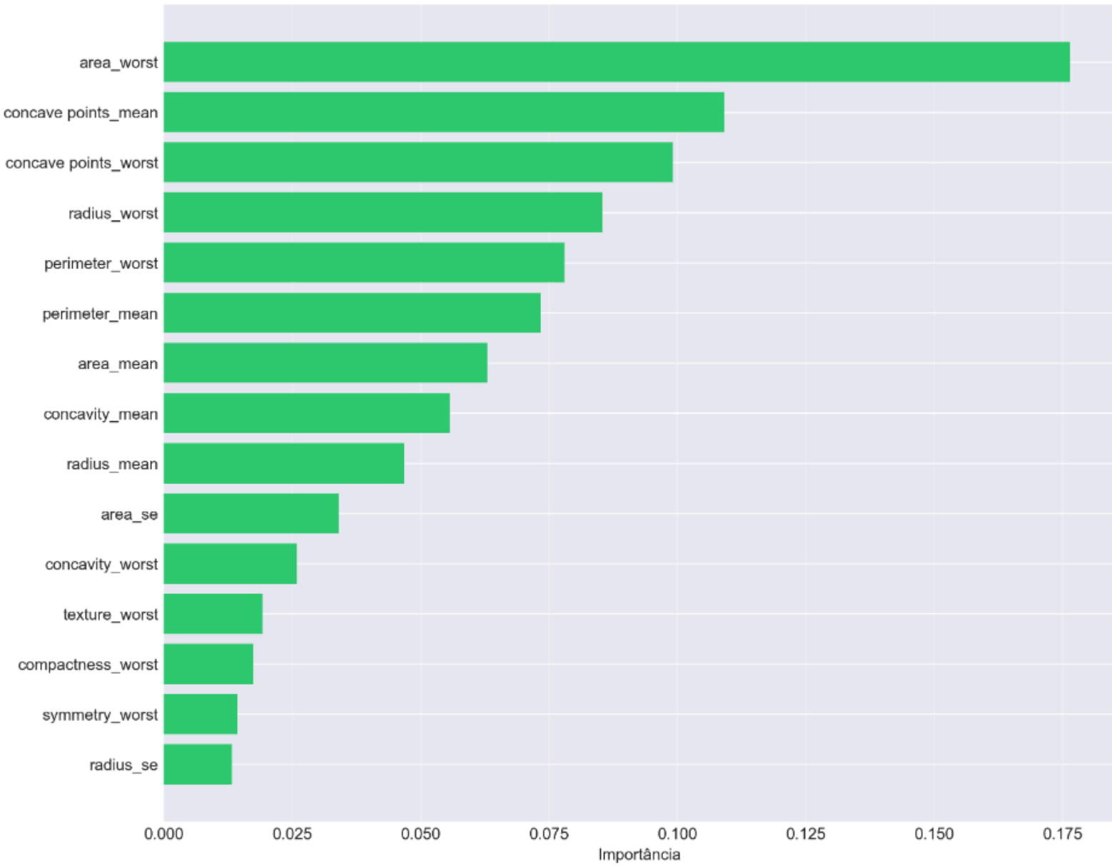
Top 15 Features - Random Forest
