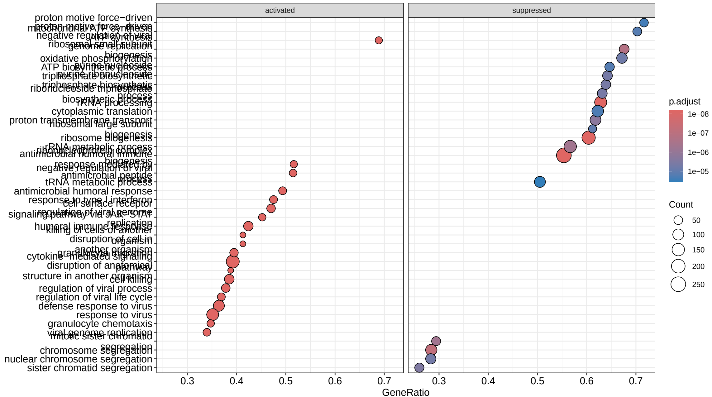
GSEA of GO Biological Process terms
