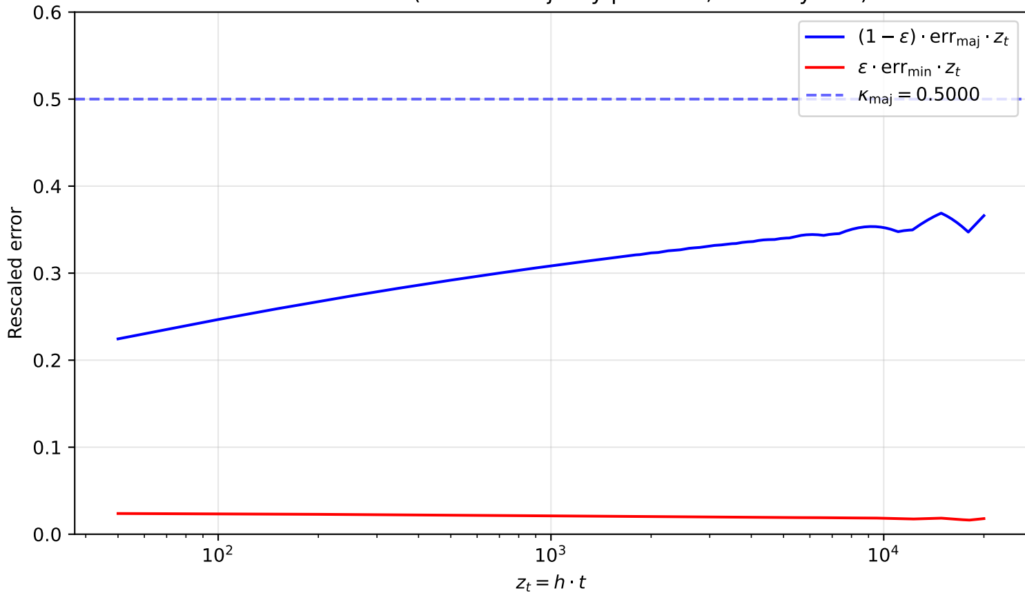
Rescaled errors ( \alpha = 1.0 : majority plateaus, minority \rightarrow 0 )
