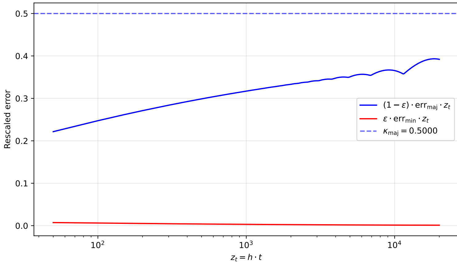
Rescaled errors ( \alpha = 1.50 > 1 : majority plateaus, minority \rightarrow 0 )
