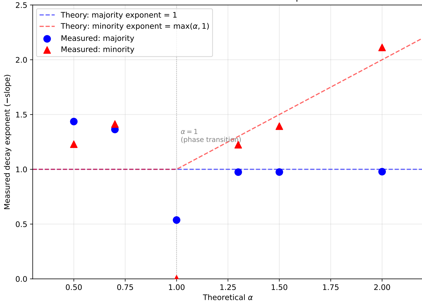
Phase transition verification: measured exponent vs. \alpha
