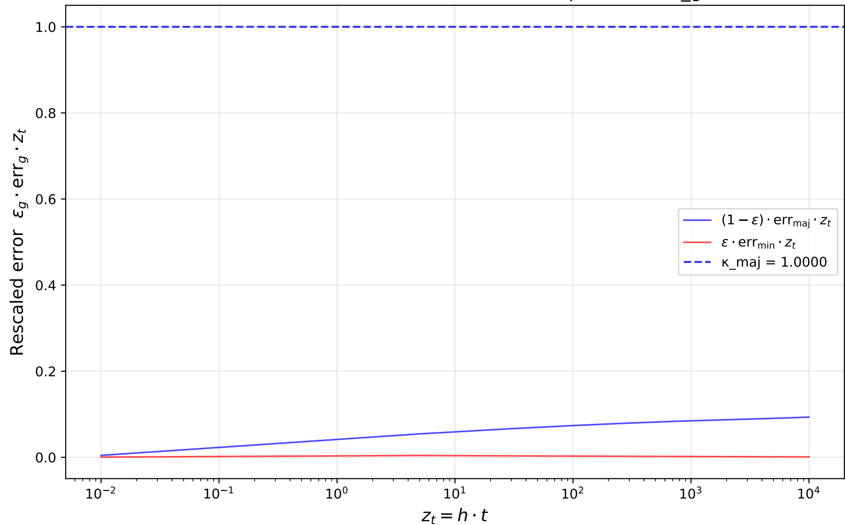
Rescaled errors — \alpha = 1.3451 (should plateau to \kappa_g )
