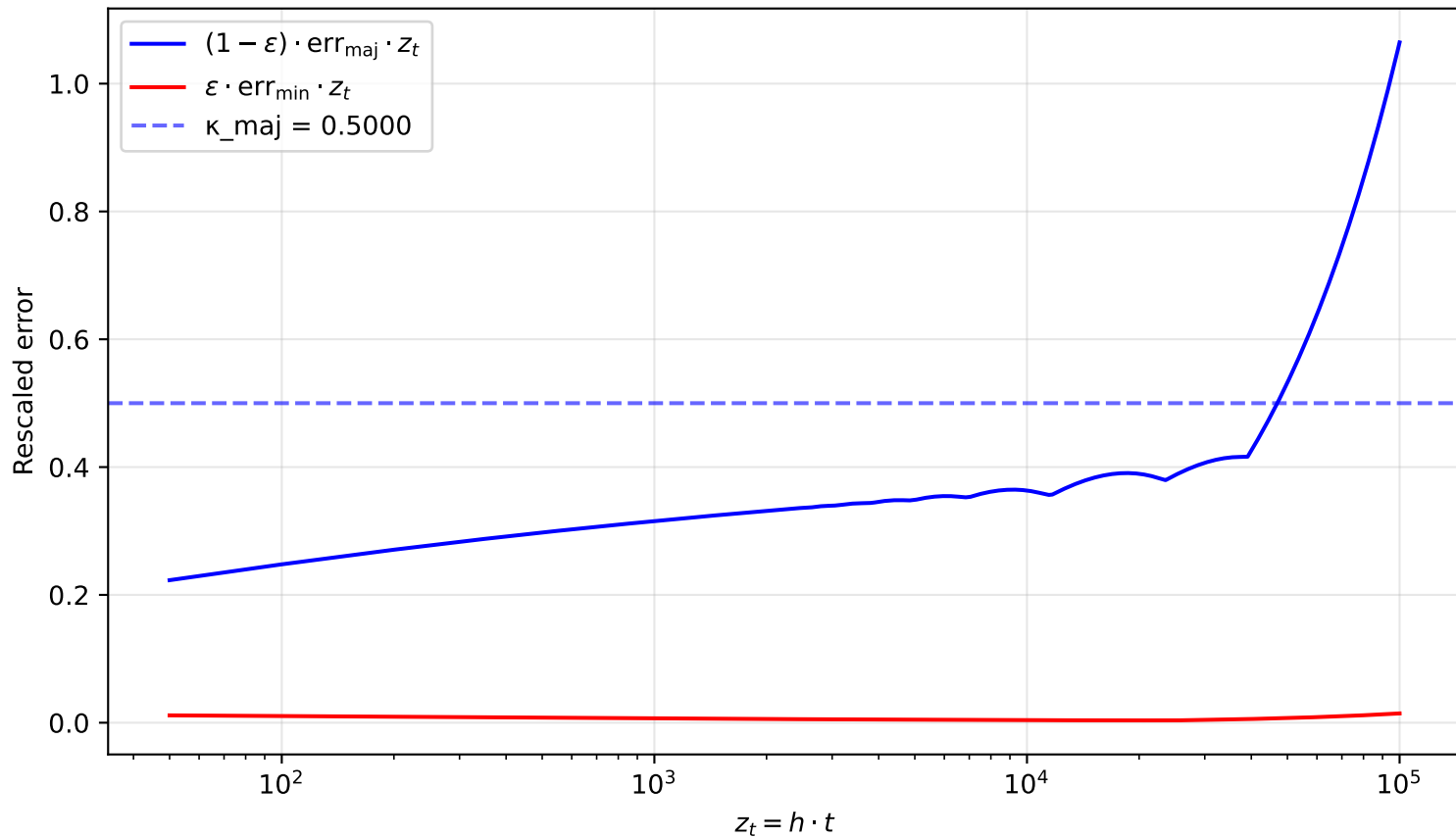
Rescaled errors ( \alpha = 1.30 > 1 : majority plateaus, minority \rightarrow 0 )
