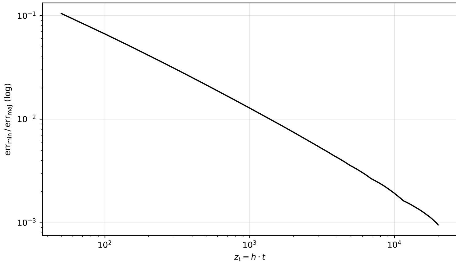
Error ratio ( \alpha = 2.00 \geq 1 : should diverge)
