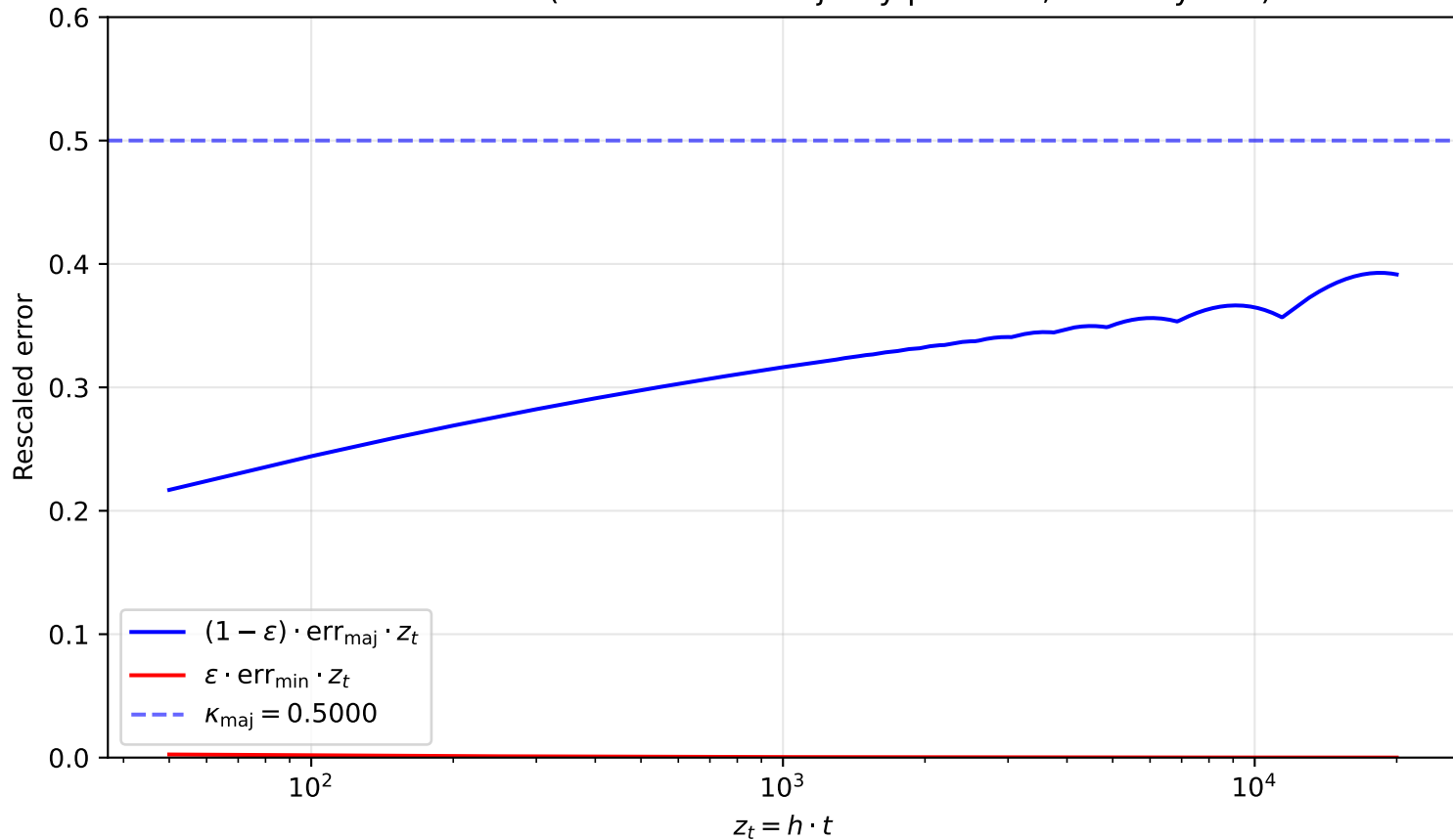
Rescaled errors ( \alpha = 2.00 > 1 : majority plateaus, minority \rightarrow 0 )
