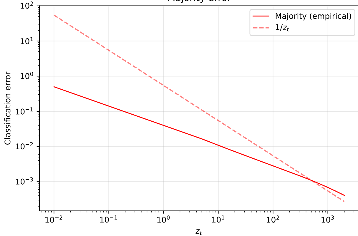
Majority error
