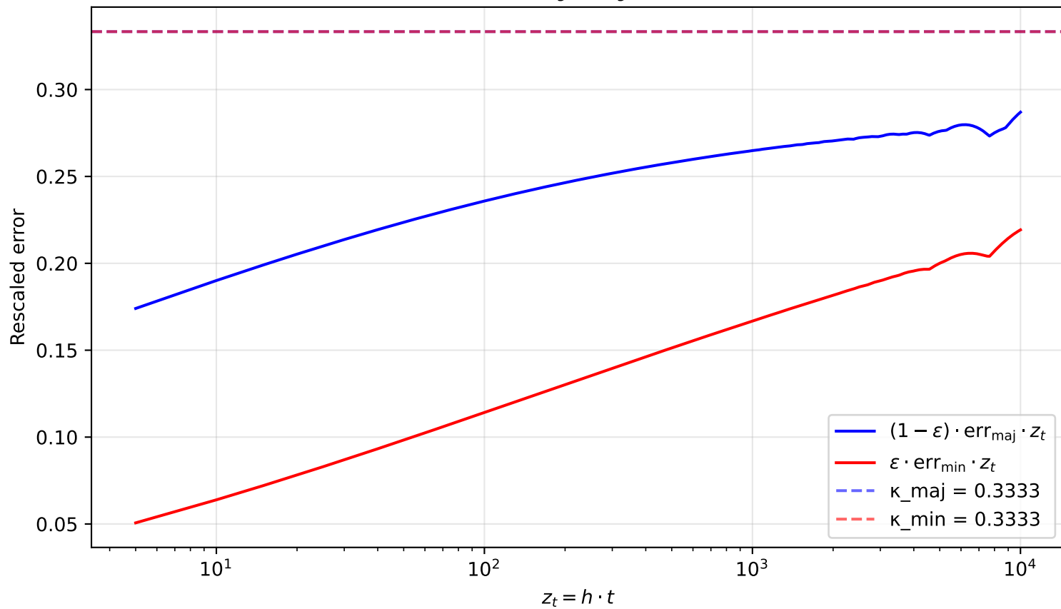
Rescaled errors \varepsilon_g \cdot \text{err}_g \cdot z_t ( \alpha = 0.50 )
