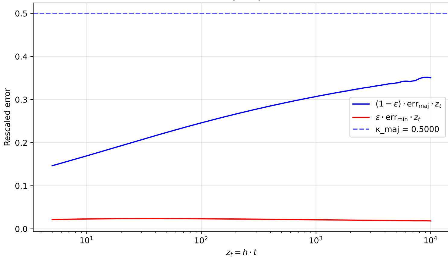
Rescaled errors \varepsilon_g \cdot \text{err}_g \cdot z_t ( \alpha = 1.00 )
