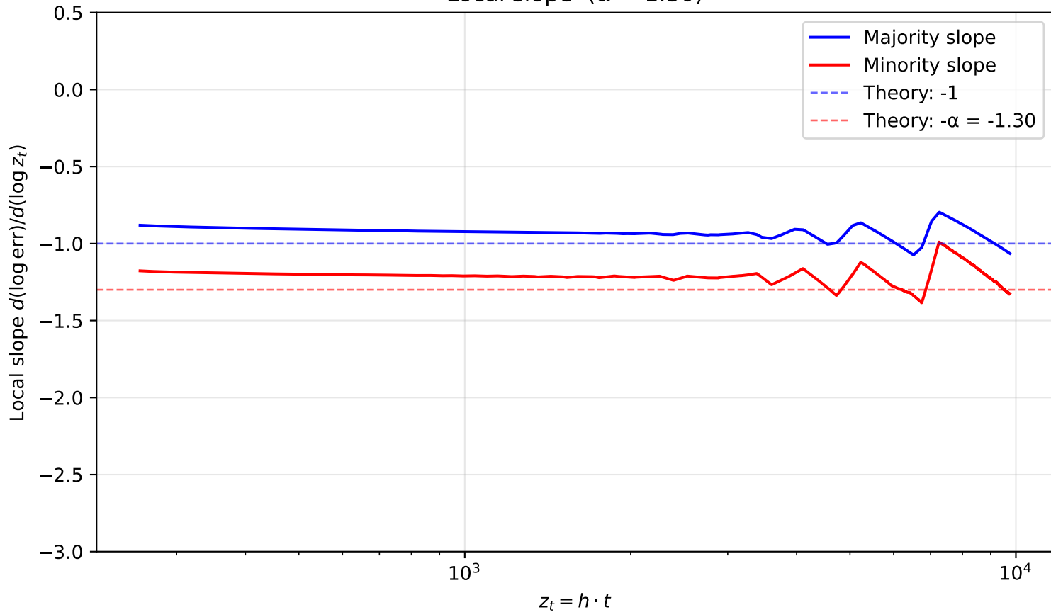
Local slope ( \alpha = 1.30 )
