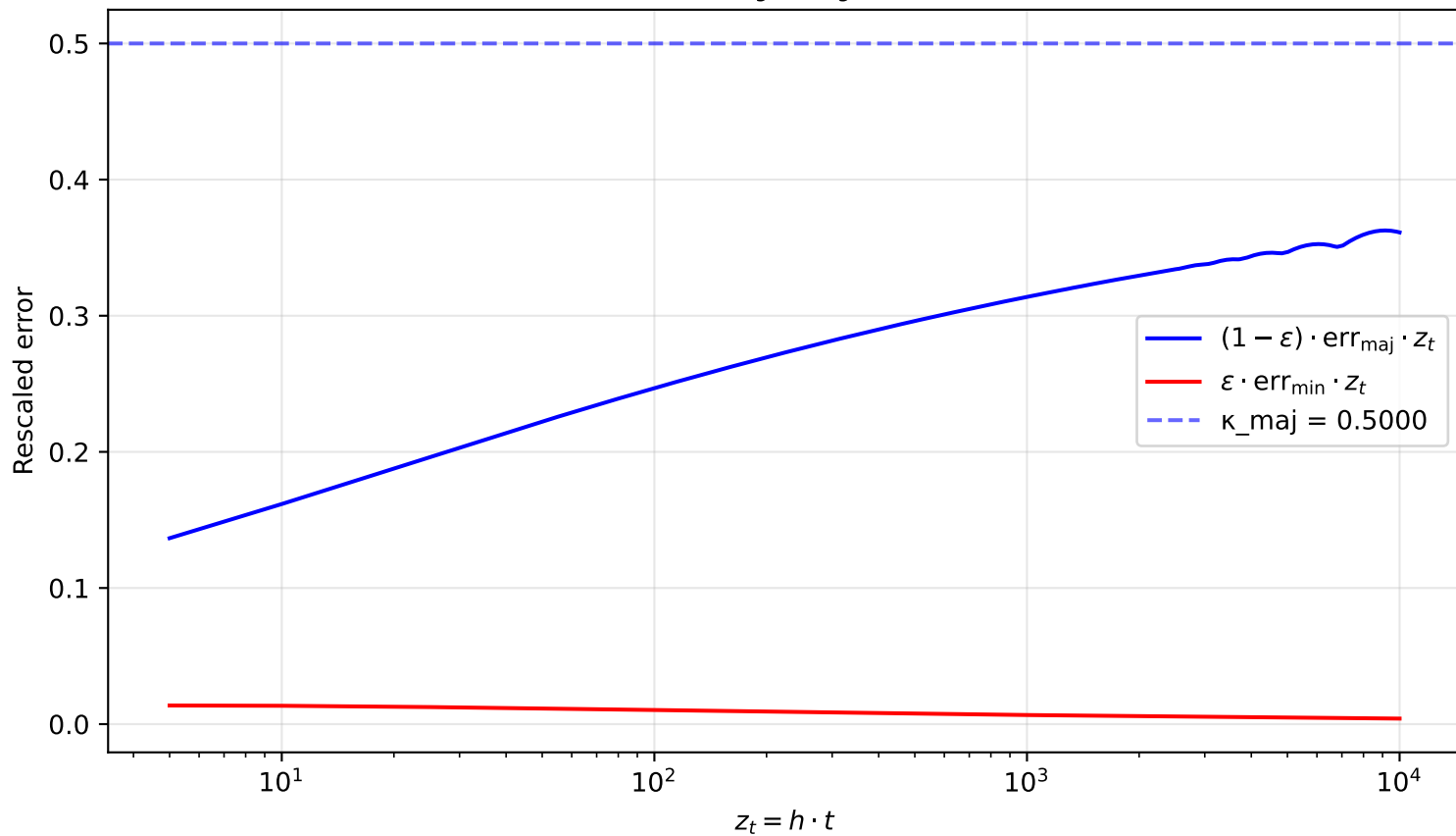
Rescaled errors \varepsilon_g \cdot \text{err}_g \cdot z_t ( \alpha = 1.30 )
