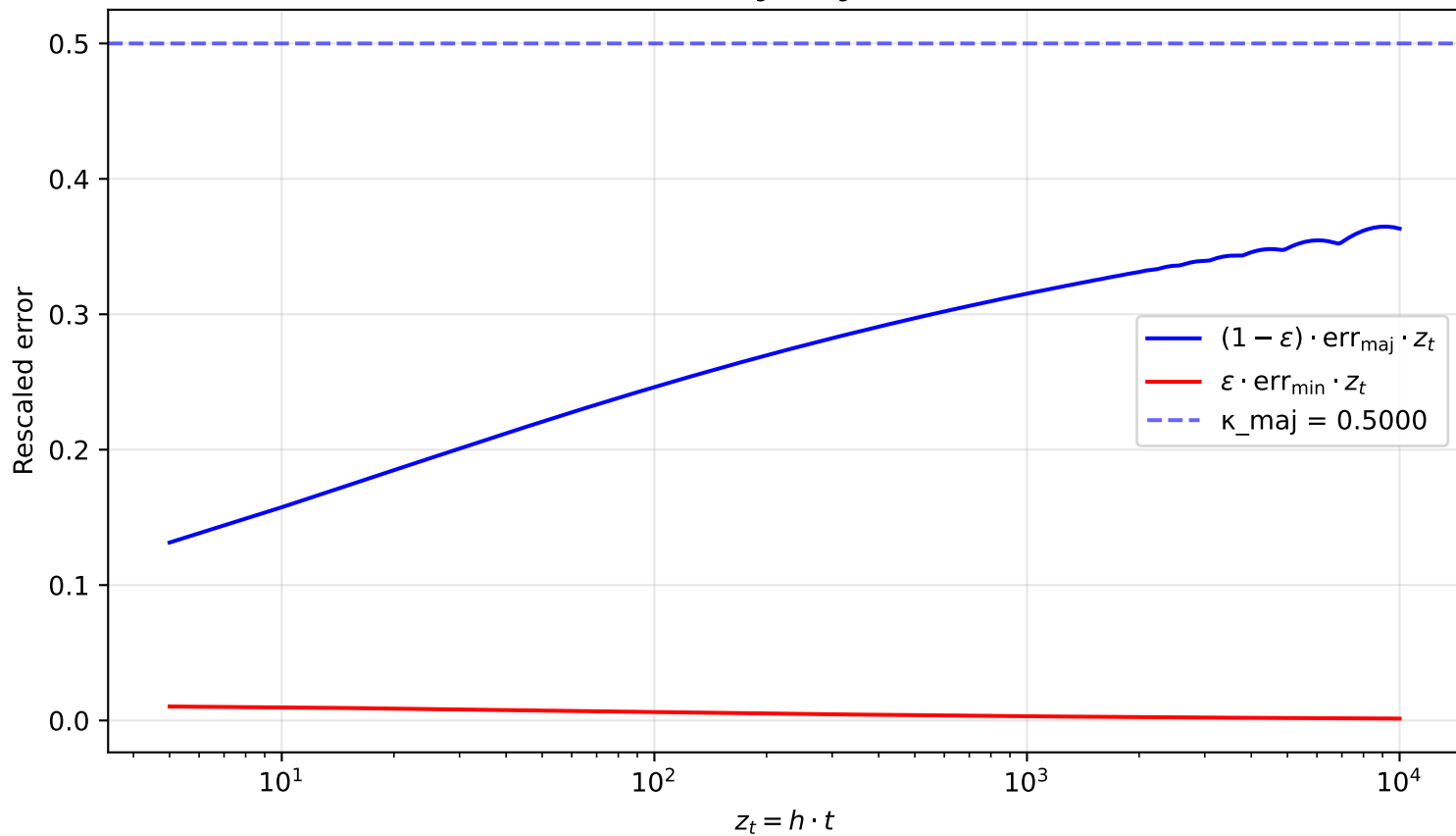
Rescaled errors \varepsilon_g \cdot \text{err}_g \cdot z_t ( \alpha = 1.50 )
