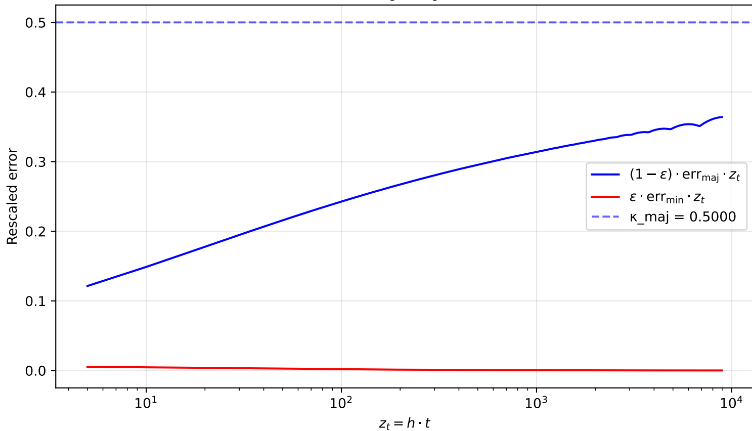
Rescaled errors \varepsilon_g \cdot \text{err}_g \cdot z_t ( \alpha = 2.00 )
