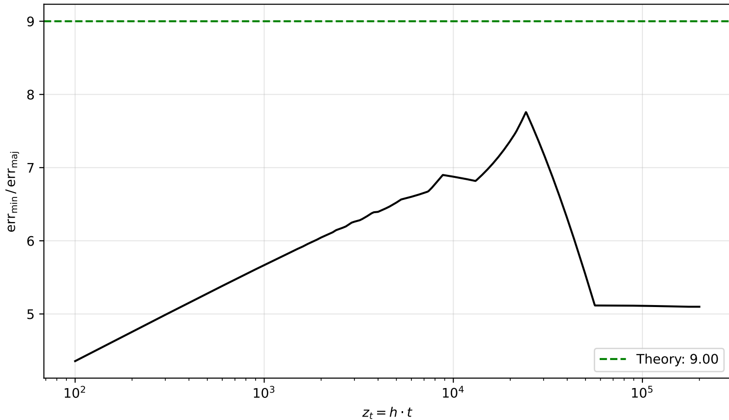
Error ratio ( \alpha = 0.50 < 1 : should converge)
