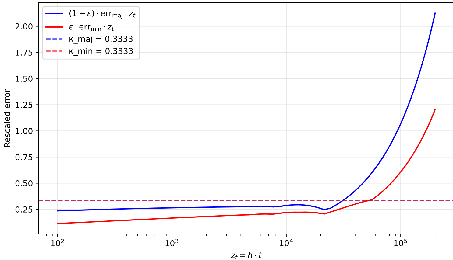
Rescaled errors ( \alpha = 0.50 < 1 : both plateau at \kappa_g )
