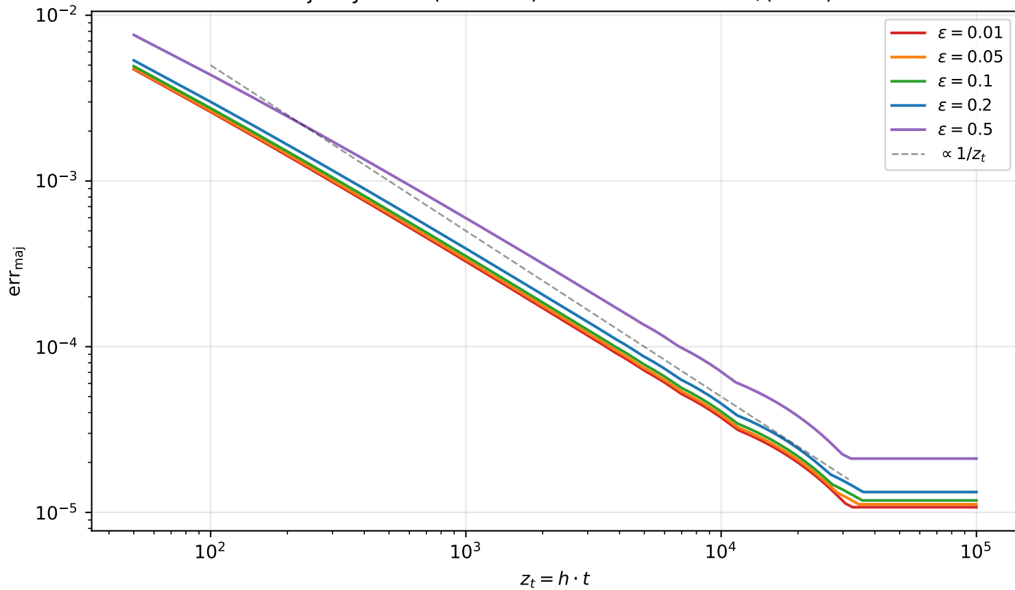
Majority error ( \alpha = 1.50 ): curves fan out \propto 1/(1 - \varepsilon)
