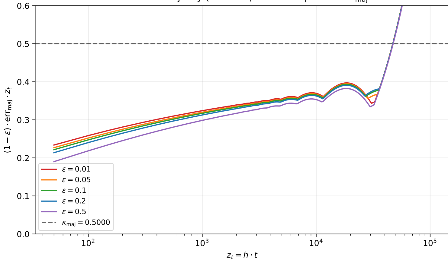
Rescaled majority ( \alpha = 1.50 ): all \varepsilon collapse onto \kappa_{\text{maj}}
