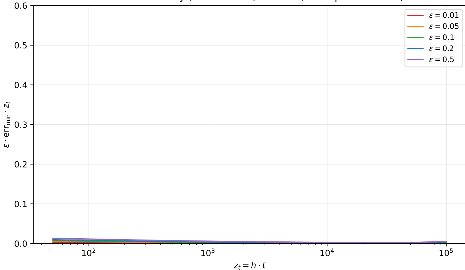
Rescaled minority ( \alpha = 1.50 \geq 1 ): all \rightarrow 0 ( \varepsilon -independent rate)
