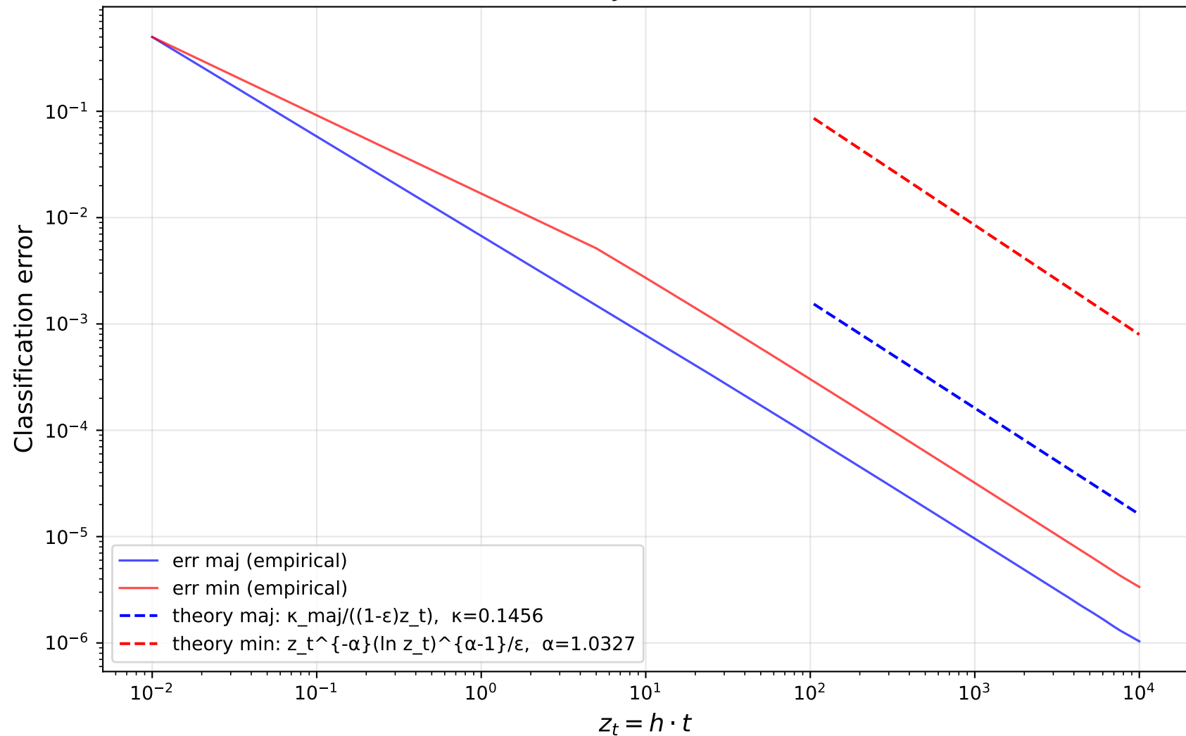
Error decay — \alpha = 1.0327
