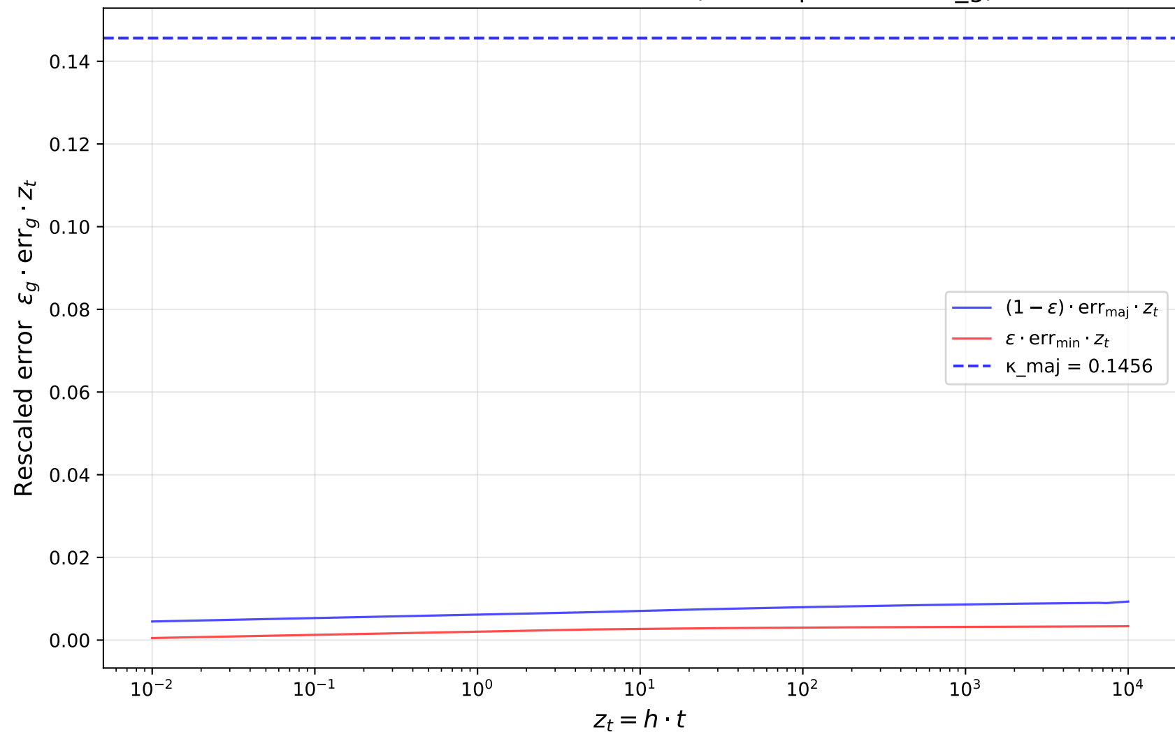
Rescaled errors — \alpha = 1.0327 (should plateau to \kappa_g )
