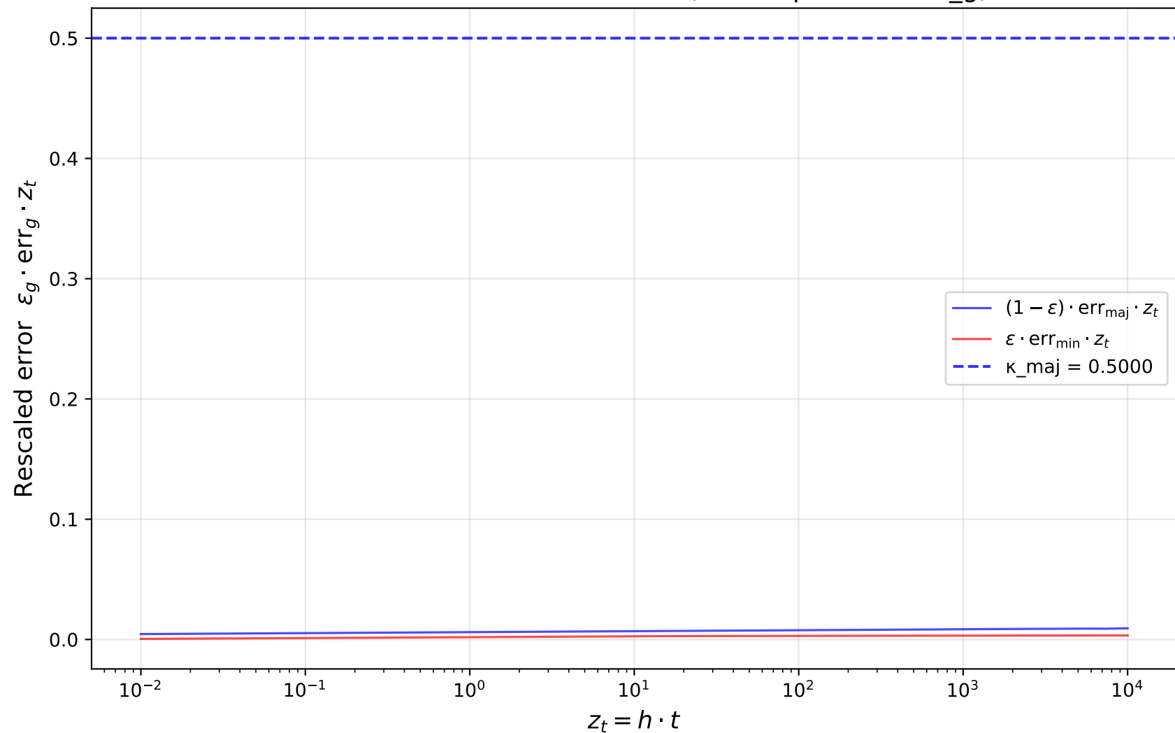
Rescaled errors — \alpha = 1.0000 (should plateau to \kappa_g )
