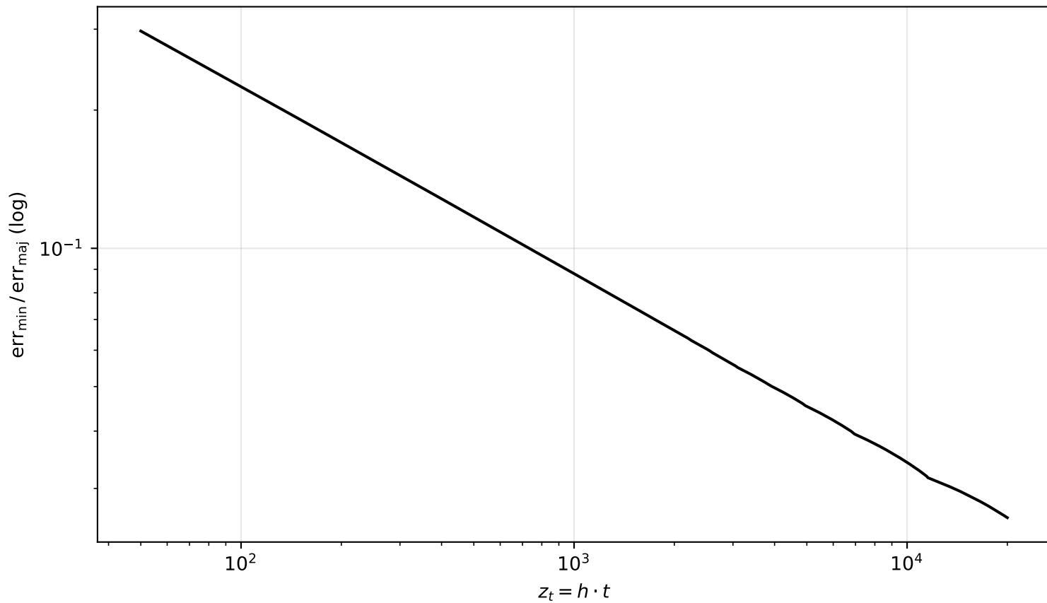
Error ratio ( \alpha = 1.50 \geq 1 : should diverge)
