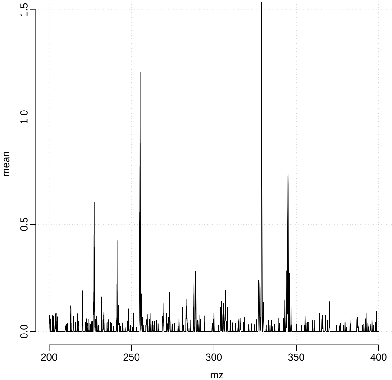
Zoomed average spectrum mean
