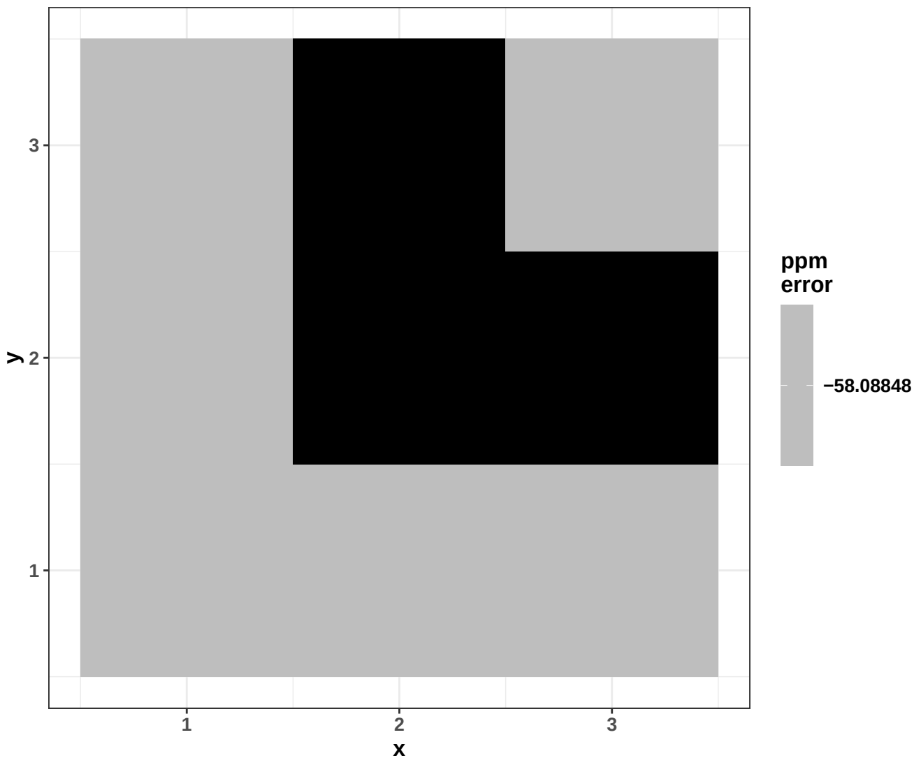
m/z accuracy for 555.1
