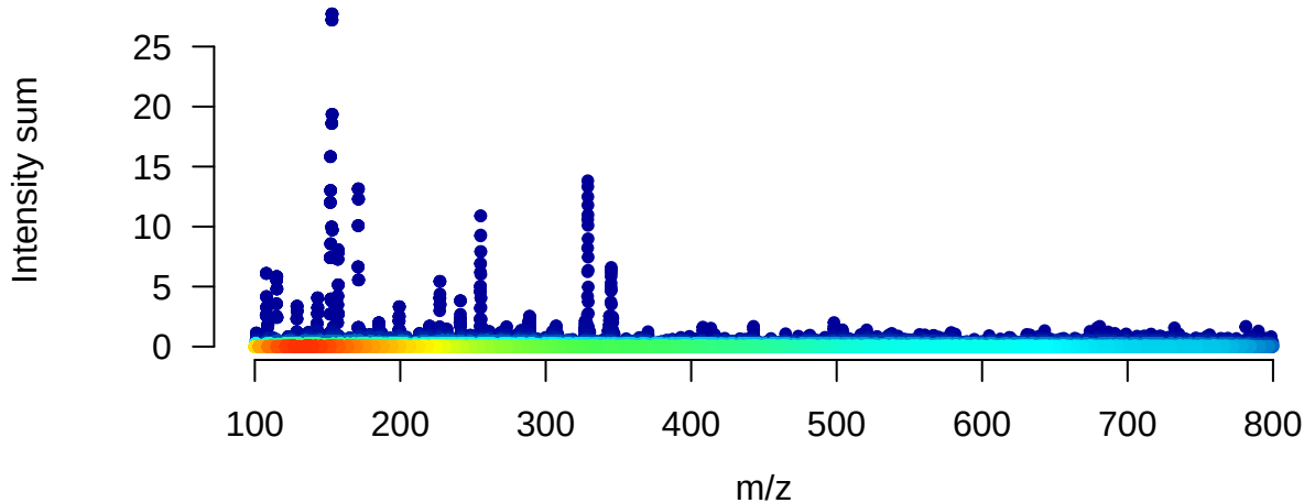
Sum of intensities per m/z
