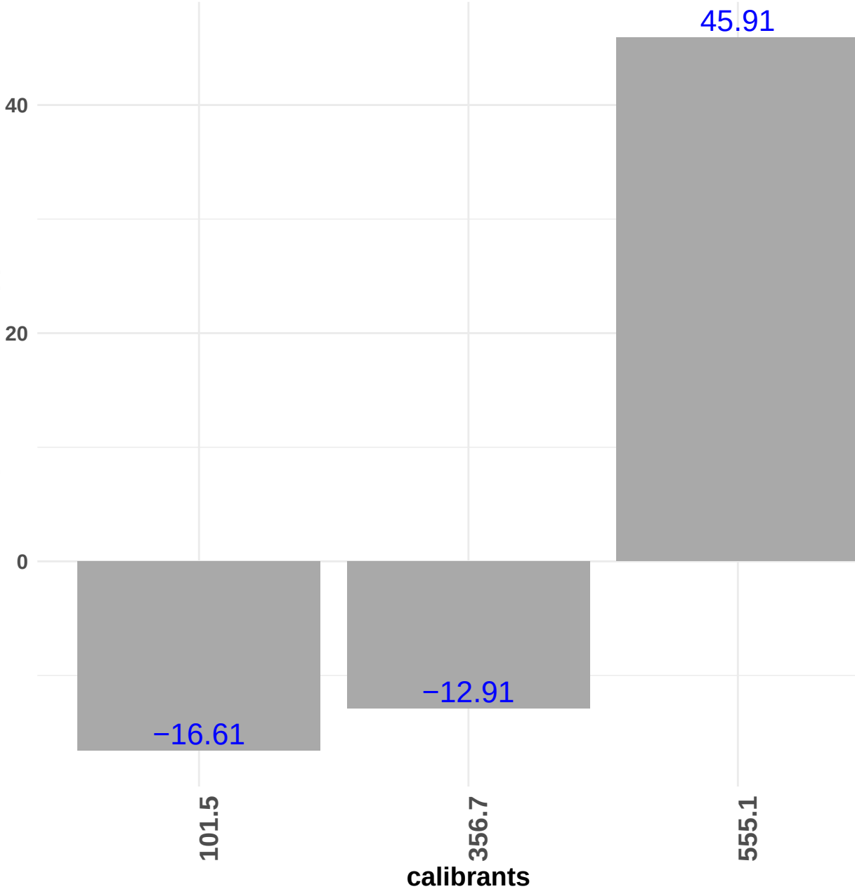
Average m/z error (closest measured m/z vs. theor. calibrant m/z)
