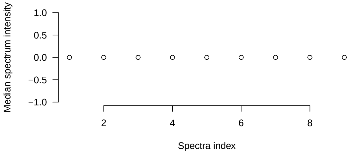
Median intensity per spectrum
