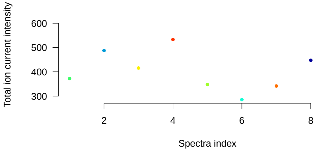
TIC per spectrum
