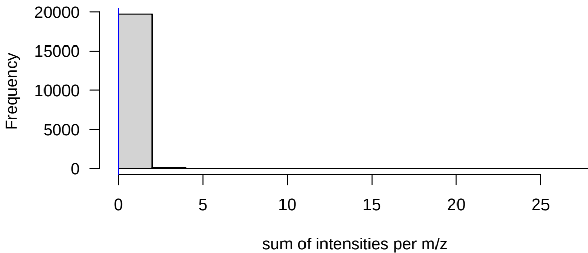
Sum of intensities per m/z
