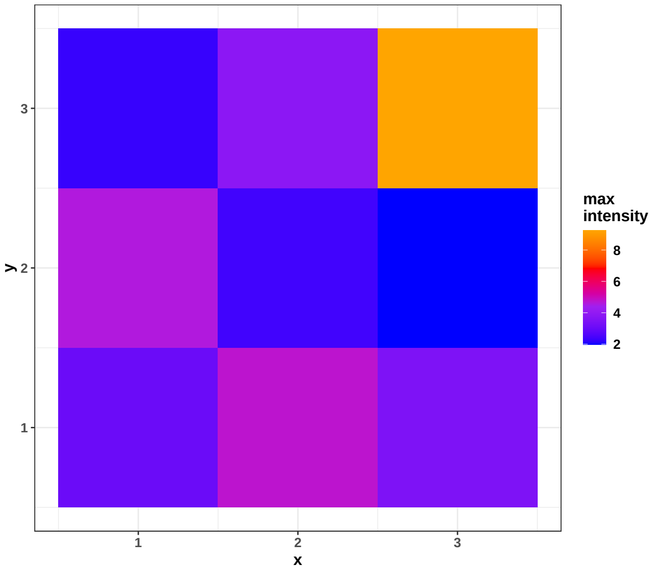
Maximum intensity per spectrum
