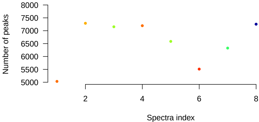
Number of peaks per spectrum
