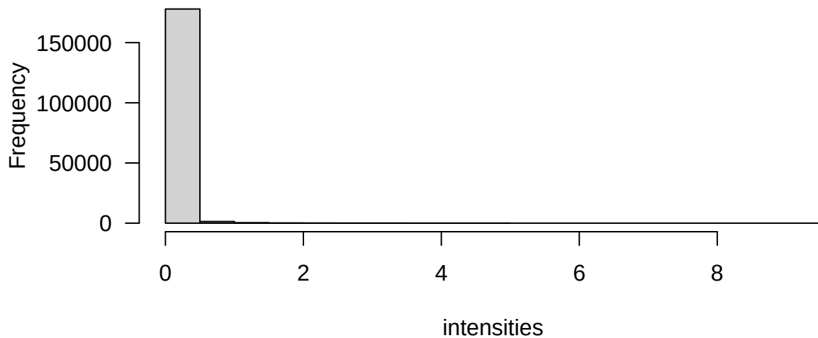
Intensity histogram
