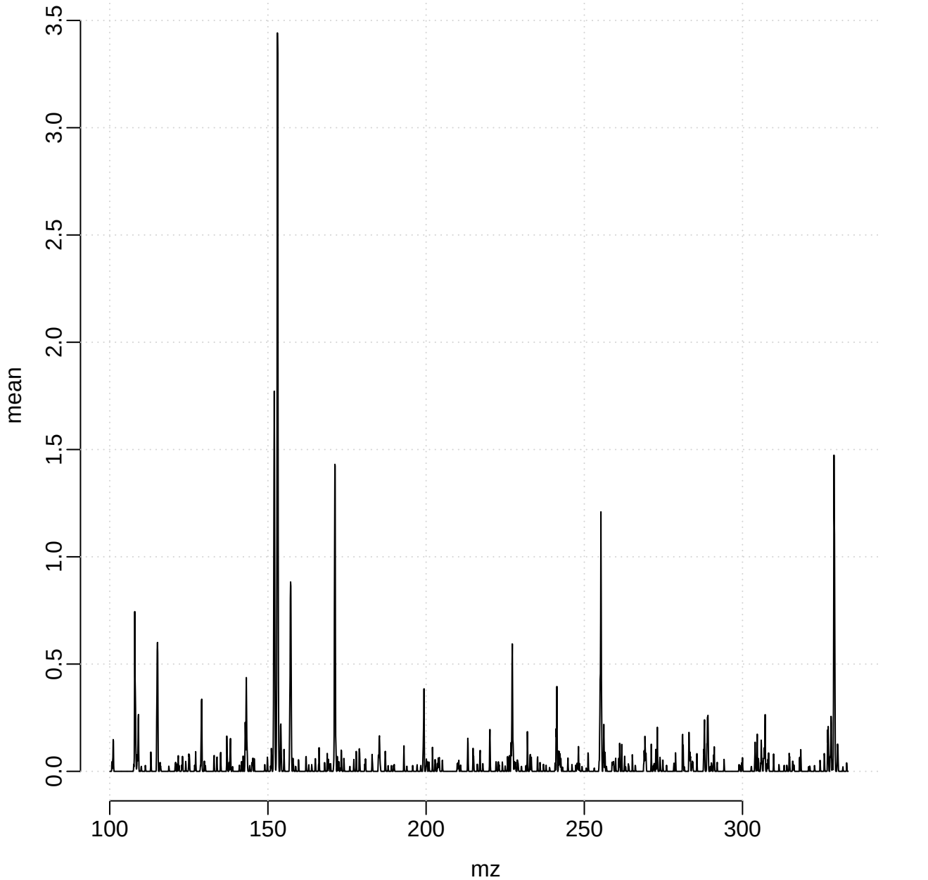
Zoomed average spectrum mean
