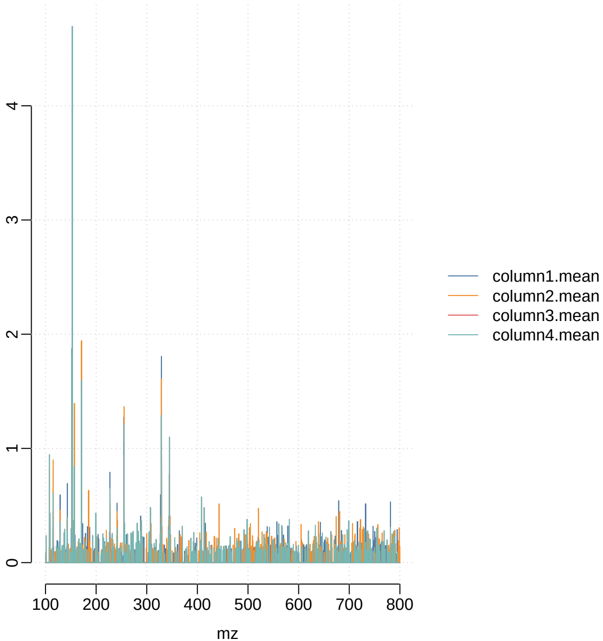
Overlaid average group spectra
