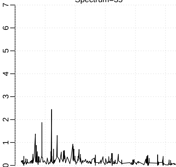
Spectrum=35
