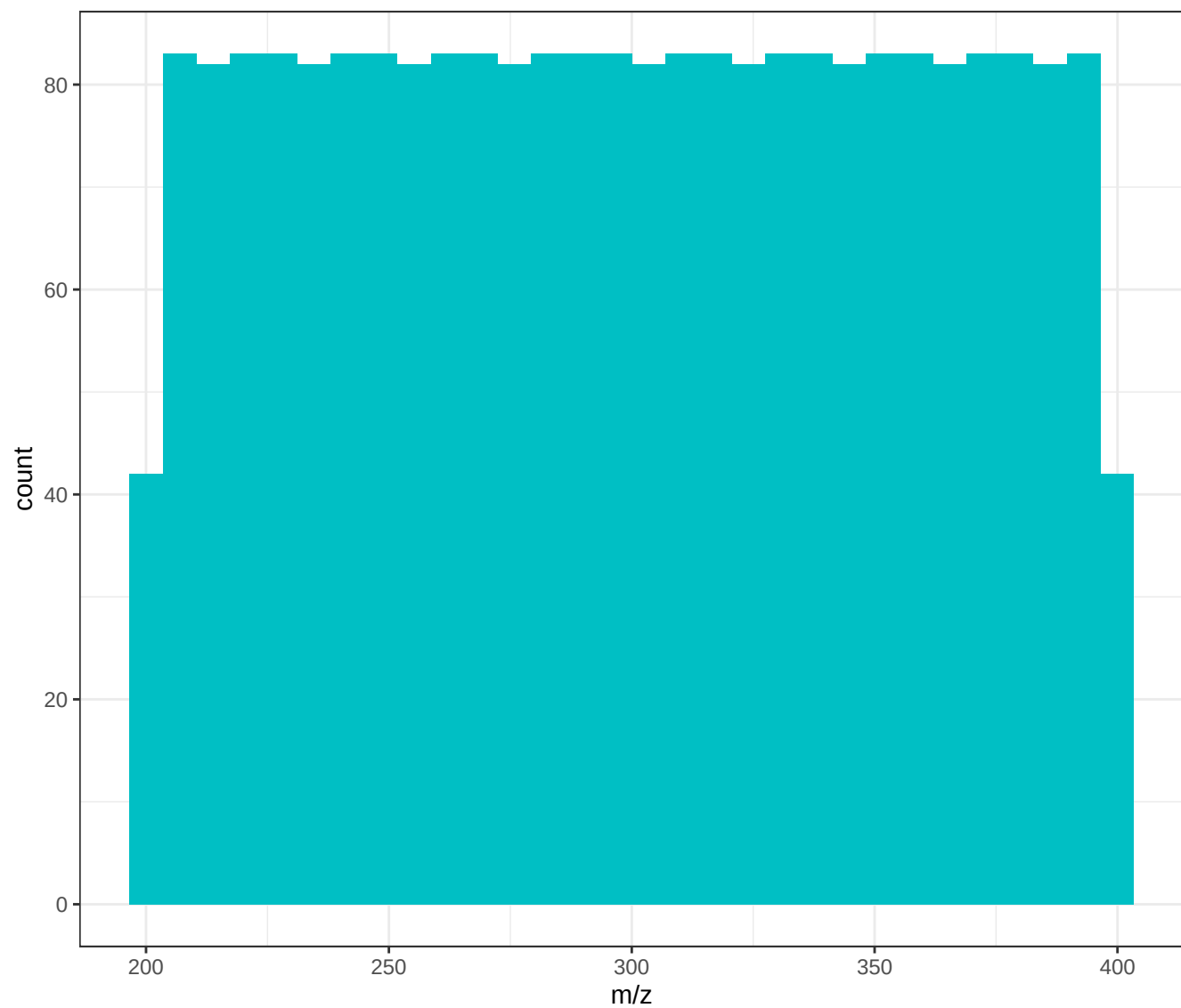
Overview of filtered m/z
